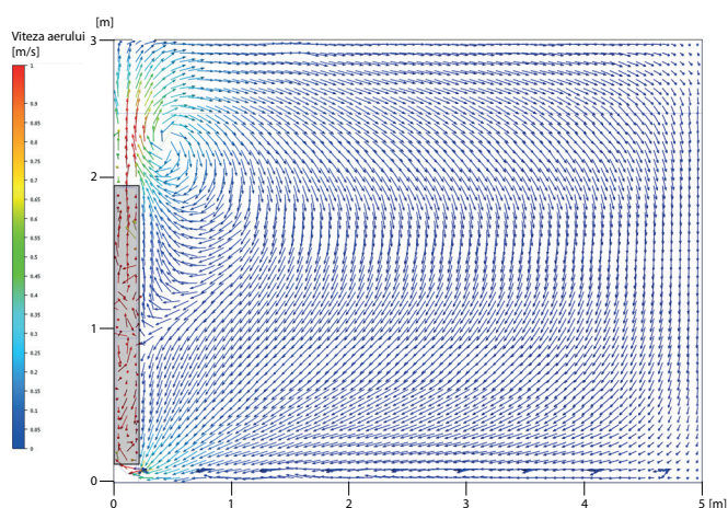
Figura 1 UV-C FiltAir
