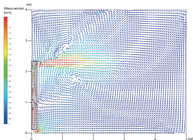
Figura 2 UV-C FiltAir-S
